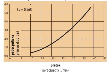
Diagram padca pritiska v vodi - DN 9, 2-stranski Pressure Drop Diagram Water - DN 9, two-way
