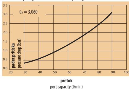
Diagram padca pritiska v vodi - DN 9, brez ventila Pressure Drop Diagram Water - DN 9, free passage
