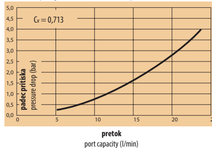
Diagram padca pritiska v vodi - DN 6, 1-stranski Pressure Drop Diagram Water - DN 6, one-way
