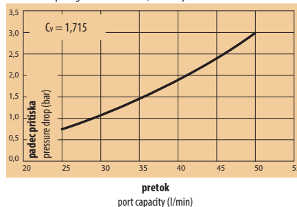
Diagram padca pritiska v vodi - DN 9, 1-stranski Pressure Drop Diagram Water - DN 9, one-way
