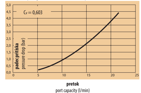
Diagram padca pritiska v vodi - DN 6, 2-stranski Pressure Drop Diagram Water - DN 6, two-way
