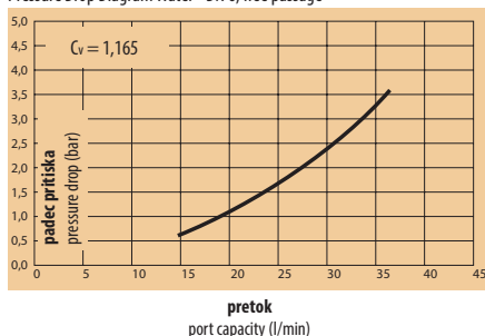
Diagram padca pritiska v vodi - DN 6, brez ventila Pressure Drop Diagram Water - DN 6, free passage
