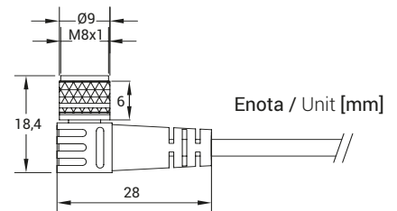
M83RL/M84RL
