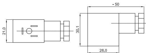
KON2224 LED.....Konektor za elektromagnete MS2224DC Connector for Solenoid Coils MS2224DC
