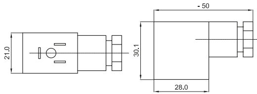
Konektor za elektromagnete MS22 Connector for Solenoid Coils MS22
